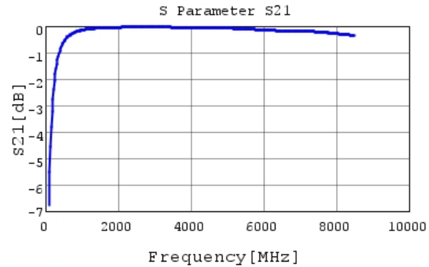
GRM1555C2A8R2CA01 S21 DCOV, 25degC
