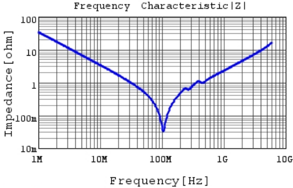
GRM2165C1H472JA01 |Z| DCOV,25degC
