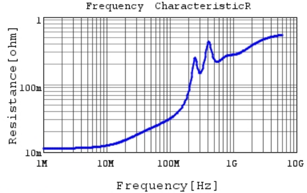
GRM2165C1H472JA01 R DCOV,25degC
