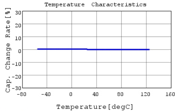
GRT0335C1E270JA02 C-Temp. capchange, DCOV, 1
