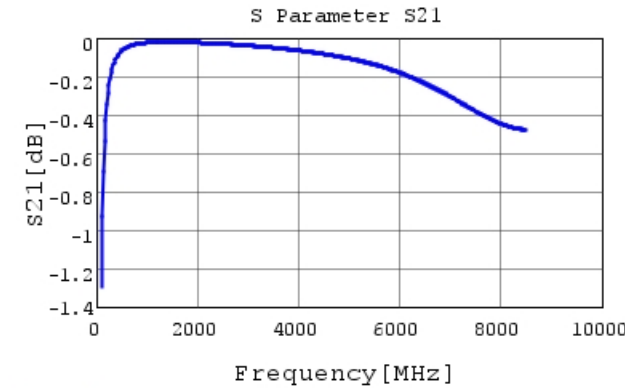
GRT0335C1E270JA02 S21 DCOV, 25degC
