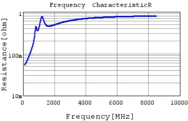
GRT1555C1H471JA02 R DCOV,25degC
