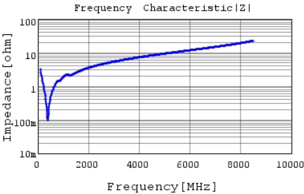
GRT1555C1H471JA02 |Z| DCOV,25degC
