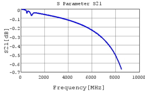
GRT1885C1E681JA02 S21 DCOV, 25degC
