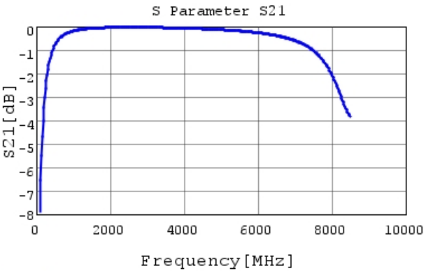
GRT1885C2A7R0DA02 S21 DCOV, 25degC
