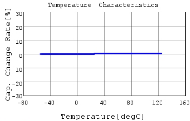
GRT1885C2A7R0DA02 C-Temp. capchange, DCOV, 1
