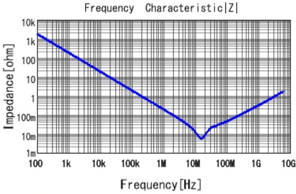
■ LLC152D70G105ME01 |Z| DCOV, 25degC
