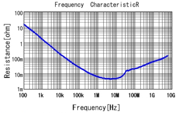
■ LLC152D70G105ME01 R DCOV, 25degC
