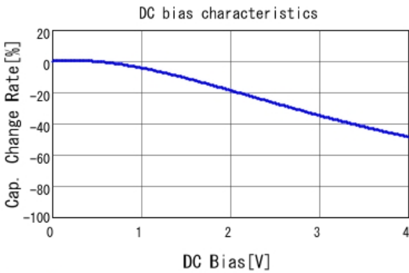
■ LLC152D70G105ME01 C-DC bias capchange, 25.0degC, A
