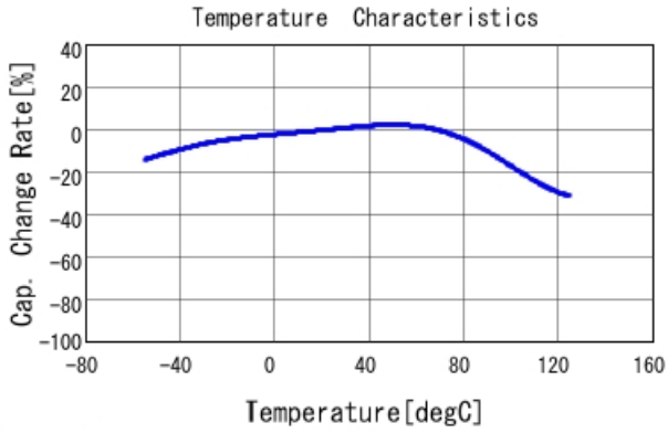
■ LLC152D70G105ME01 C-Temp. capchange, DC0.0V, AC0.1
