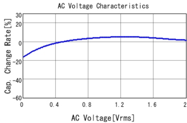
■ LLC152D70G105ME01 C-AC Voltage capchange, DCOV, 25
