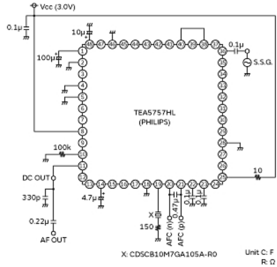
Measurement Circuit
