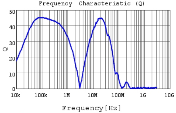
B1047AS-471M Q
