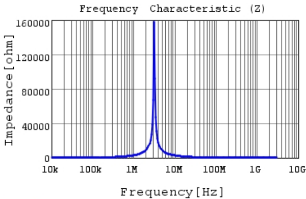
B1047AS-471M |Z|
