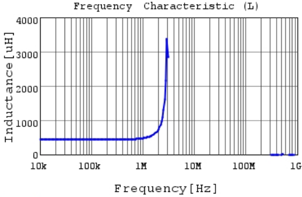
B1047AS-471M L
