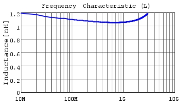
LQG15HZ1N1B02 L
