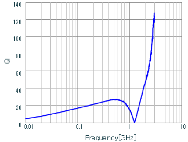
LQG15WZR11J02 Q.
