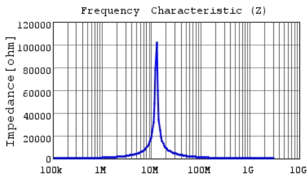
LQH32NH121J23 |Z|
