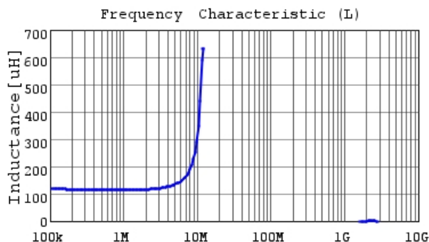
LQH32NH121J23 L
