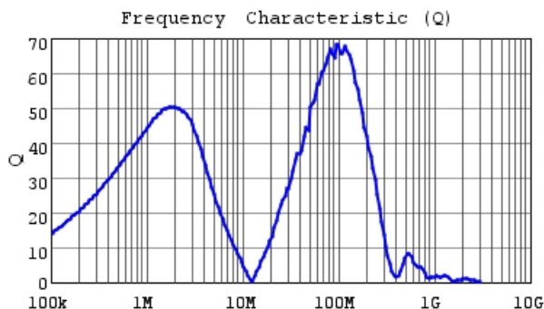
LQH32NH121J23 Q
