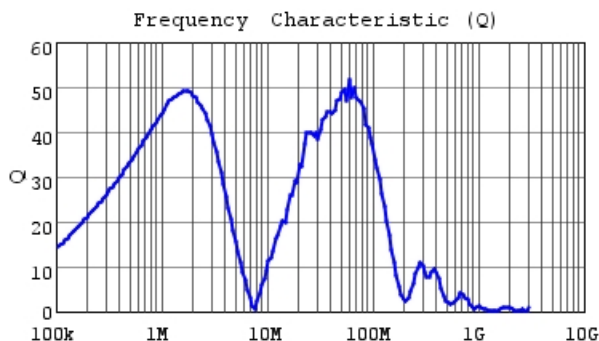
LQH32NH331J23 Q
