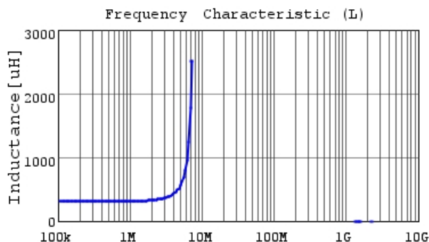
LQH32NH331J23 L
