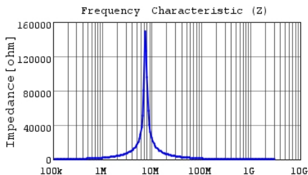
LQH32NH331J23 |Z|
