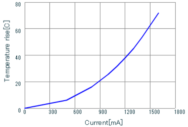
LQH32PN3R3NN0 DT_Current
