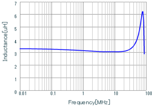
LQH32PN3R3NN0 L
