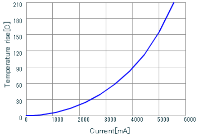
LQH3NPZR47NGR DT_Current
