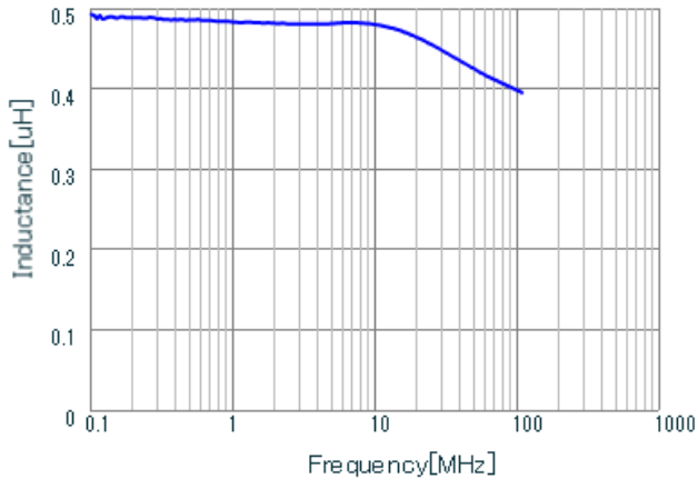
LQH3NPZR47NGR L
