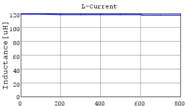
LQM18JNR12J00 L-Current 20degC
