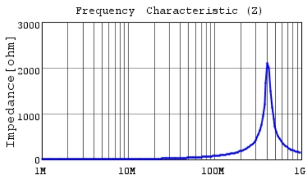
LQM18JNR12J00 |Z|
