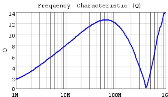
LQM18JNR12J00 Q
