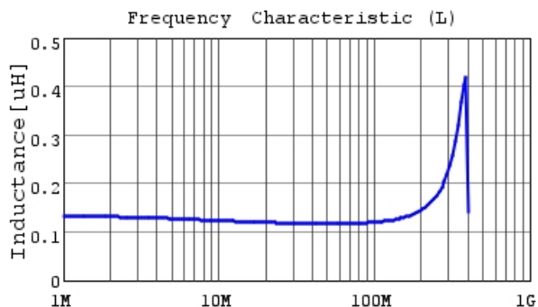
LQM18JNR12J00 L
