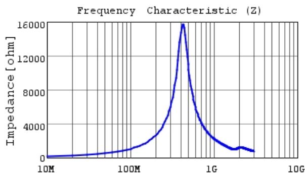
LQW21HN1R5J00 |Z|
