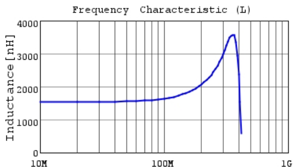
LQW21HN1R5J00 L
