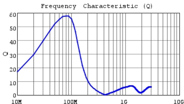
LQW21HN1R5J00 Q
