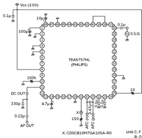
Measurement Circuit
