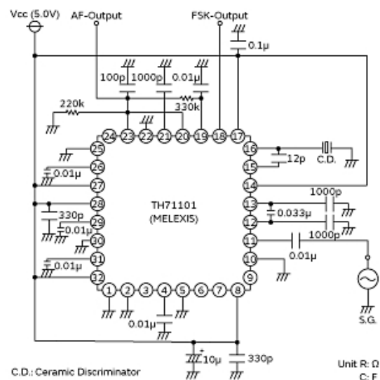
Measurement Circuit
