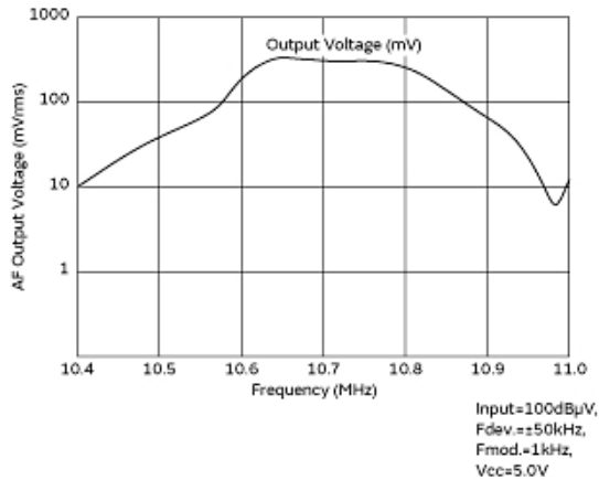
Frequency Characteristics
