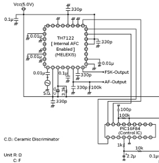
Measurement Circuit
