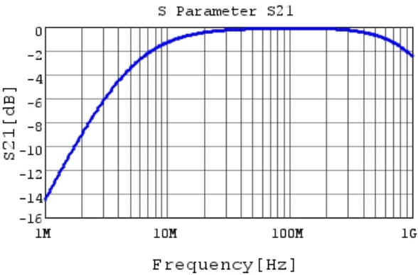
DE1B3RA331KA4BQ01F S21 DCOV, 20degC
