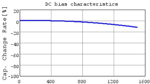
DE1B3RB101KJ4BR01F C-DC bias capchange, 20.0
