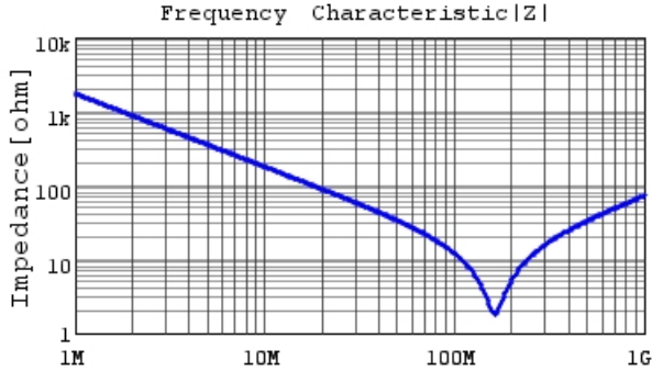
DE1B3RB101KJ4BR01F |Z| DCOV, 20degC
