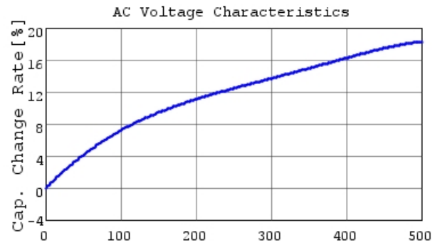
DE1B3RB101KJ4BR01F C-AC Voltage capchange, 1
