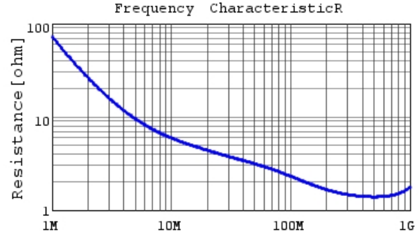
DE1B3RB101KJ4BR01F R DCOV, 20degC
