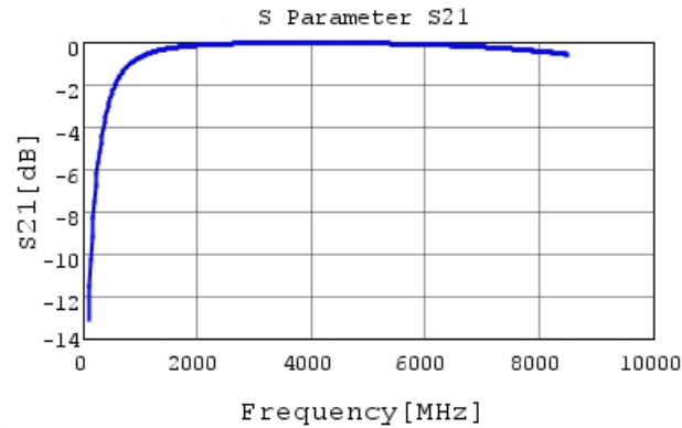
GRM1555C1H3R6CA01 S21 DCOV, 25degC
