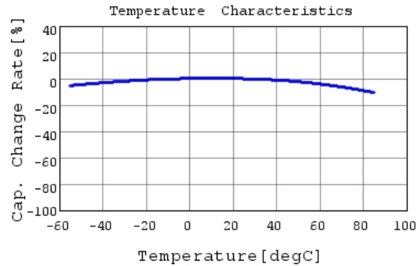
GRM155R60J224KE01 C-Temp. capchange, DC0.0V,
