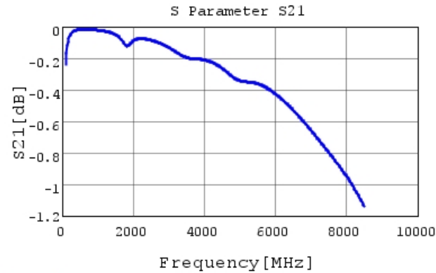
GRM1885C2A680JA01 S21 DCOV, 25degC
