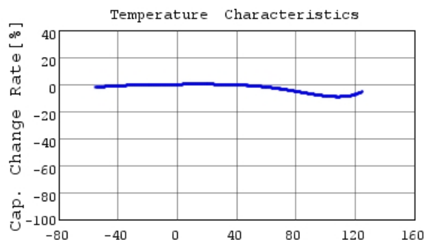
GRM188R71H331KA01 C-Temp. capchange, DC0.0V,
