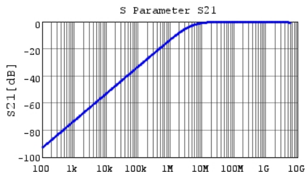
GRM188R71H331KA01 S21 DC0V,25degC
