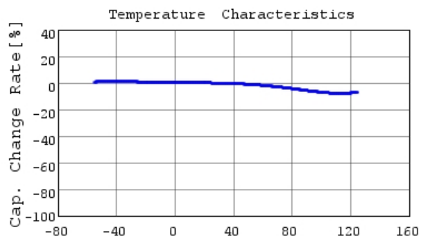
GRM21BR71H154KA01 C-Temp. capchange, DC0.0V,
