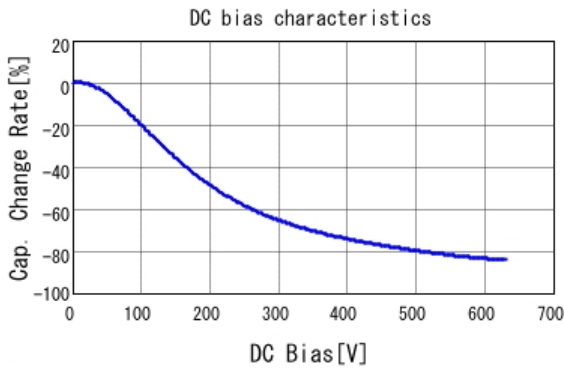
■ RDER72J474MUB1H03B C-DC bias capchange, 25.0degC, AC1
