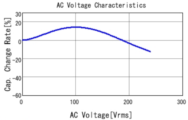
RDER72J474MUB1H03B C-AC Voltage capchange, DC0V, 2
