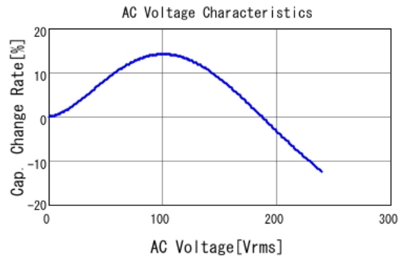
■ RDER72J474MUB1H03B C-AC Voltage capchange, DC0V, 25.0
