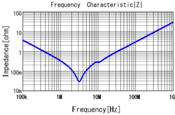
RDER72J474MUB1H03B |Z| DC0V, 25degC
