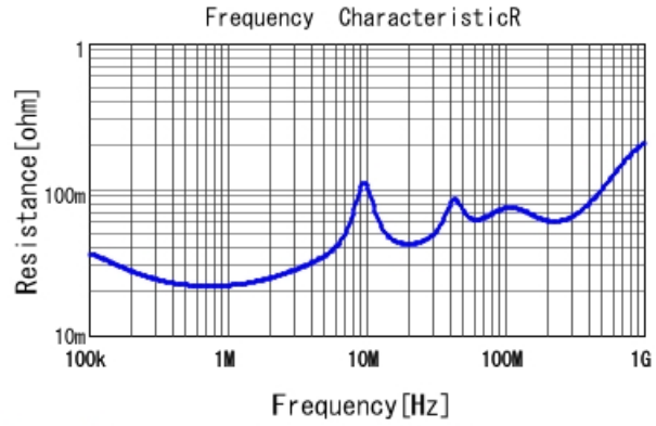
RDER72J474MUB1H03B R DC0V, 25degC
