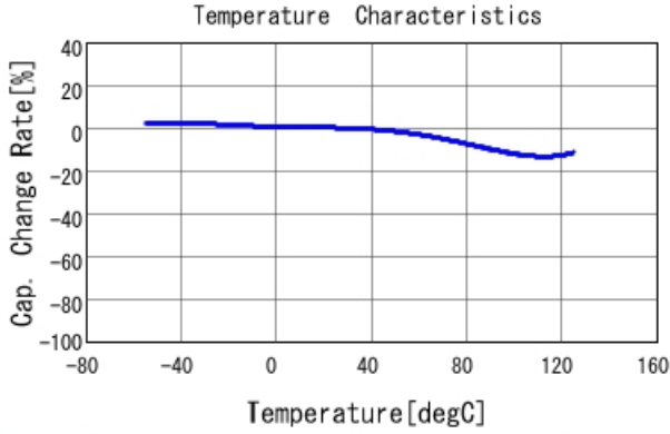
RDER72J474MUB1H03B C-Temp. capchange, DCOV, AC1Vrr
