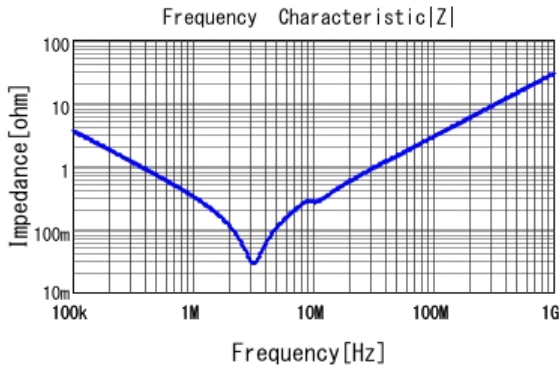
■ RDER72J474MUB1H03B |Z| DC0V, 25degC
