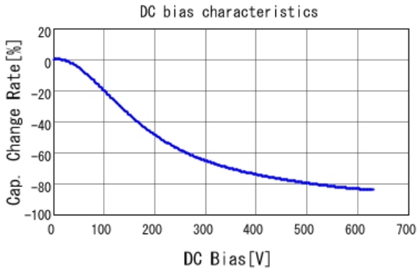
RDER72J474MUB1H03B C-DC bias capchange, 25.0degC,
