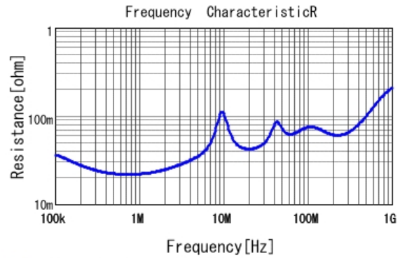
■ RDER72J474MUB1H03B R DC0V, 25degC
