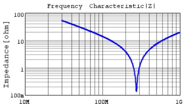
RHE5G1H101J0DBH03A |Z| DCOV,25degC
