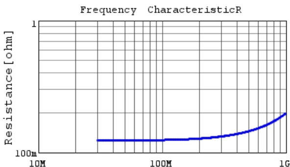
RHE5G1H101J0DBH03A R DCOV,25degC
