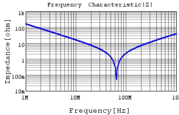
RHE5G1H102J0K1H03B |Z| DCOV, 25degC
