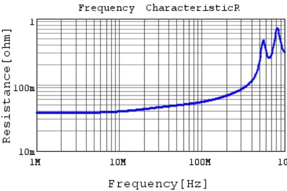
RHE5G1H102J0K1H03B R DCOV, 25degC
