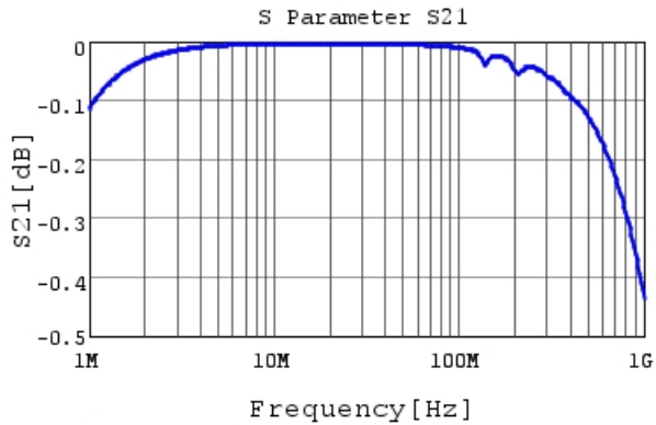
RHE5G1H103J1K1H03B S21 DCOV, 25degC
