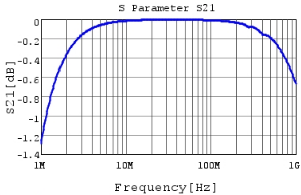
RHE5G1H272J0M1H03A S21 DCOV, 25degC
