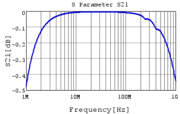
RHE5G1H472J1M1H03A S21 DCOV, 25degC
