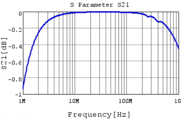
RHE5G2A332J1M1H03A S21 DCOV, 25degC
