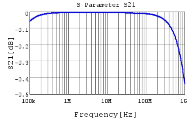
RHEL81H154K1K1H03B S21 DCOV, 25degC
