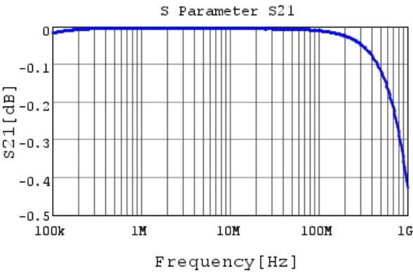
RHEL81H334K1M1H03A S21 DCOV, 25degC
