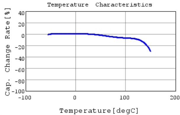
RHEL81H334K1M1H03A C-Temp. capchange, DCOV,
