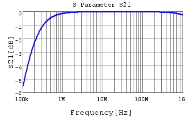
RHEL82A103K0DBH03A S21 DCOV, 25degC
