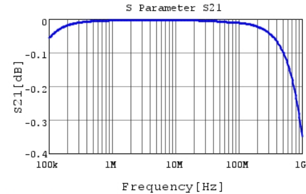
RHEL82A154K2DBH03A S21 DCOV, 25degC
