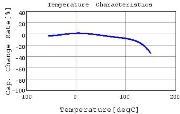
RHEL82A154K2DBH03A C-Temp. capchange, DCOV,
