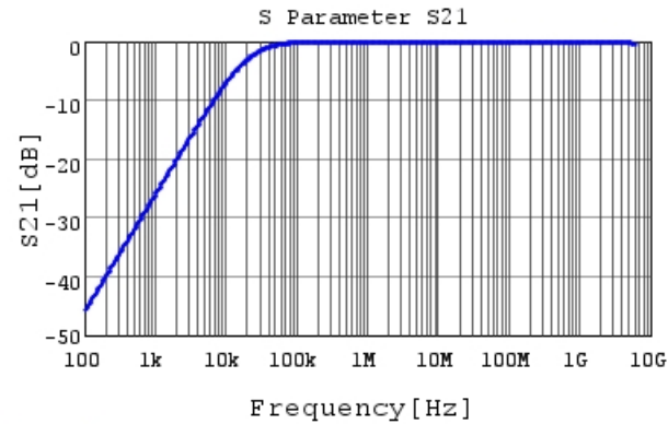
GCJ188R71E823KA12 S21 DC0V,25degC
