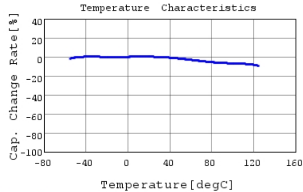
GCJ188R71E823KA12 C-Temp. capchange, DC0.0V,
