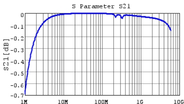
Frequency [Hz] GCM1885C1H392JA16 S21 DCOV, 25degC
