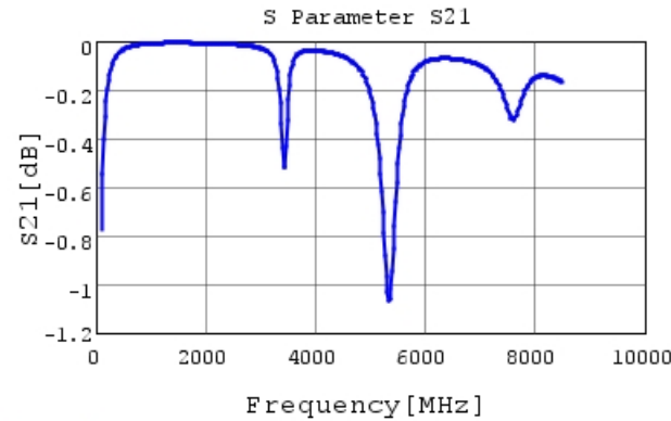
GCQ1555C1H360JB01 S21 DCOV, 25degC
