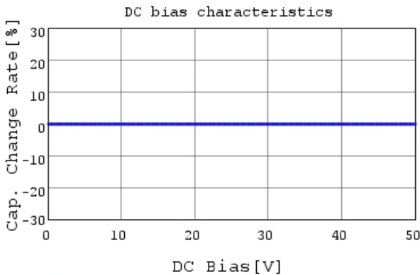
GJM1555C1H100FB01 C-DC bias capchange, 25.0C
