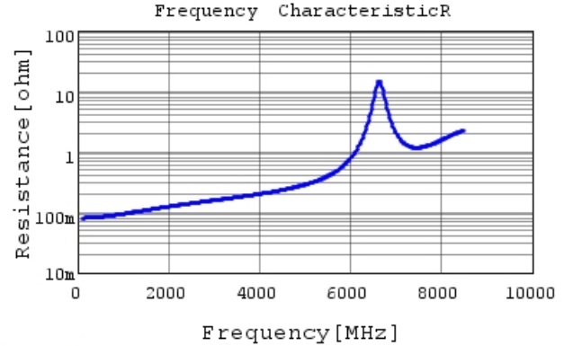
GJM1555C1H100FB01 R DCOV, 25degC
