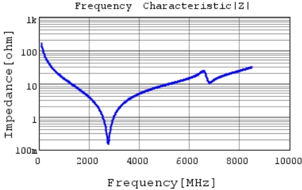
GJM1555C1H100FB01 |Z| DCOV, 25degC
