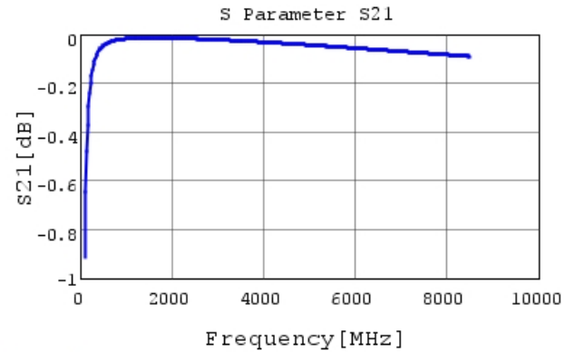
GRM0115C1C330JE01 S21 DCOV, 25degC
