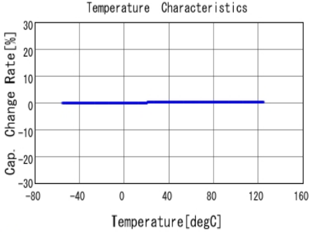
■ GRM0223C1H2R3BA03 C-Temp. capchange, DCOV, AC1Vrms
