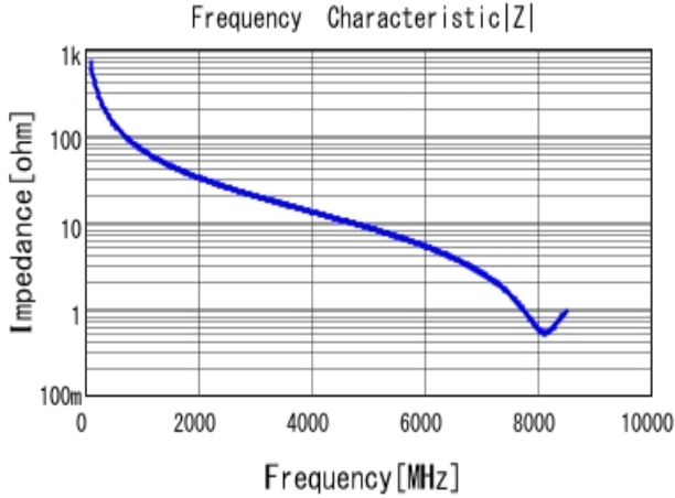
■ GRM0223C1H2R3BA03 |Z| DCOV, 20degC
