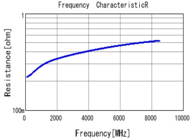
■ GRM0223C1H2R3BA03 R DCOV, 20degC
