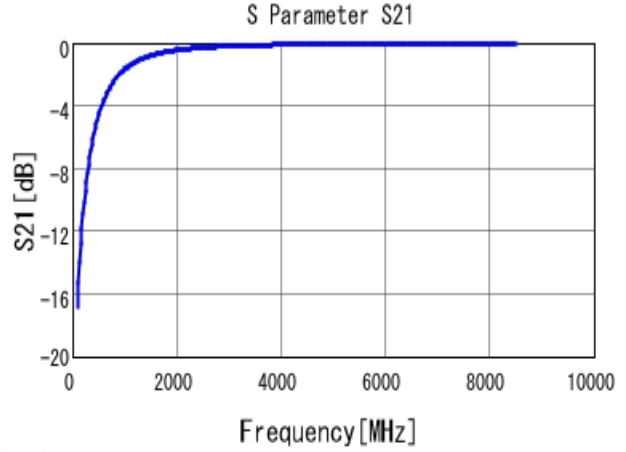
■ GRM0223C1H2R3BA03 S21 DCOV, 20degC
