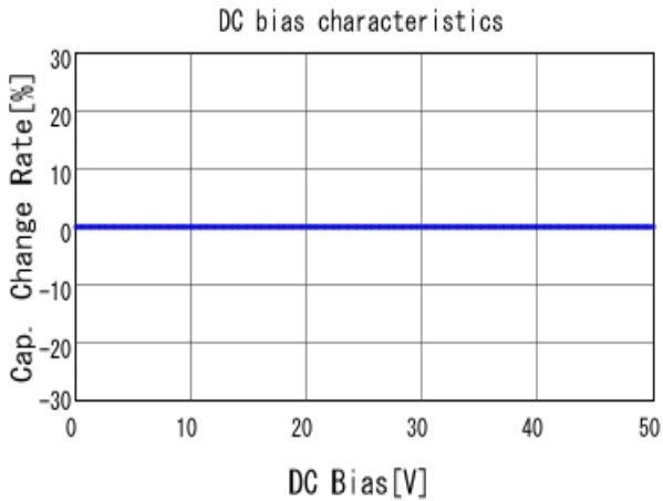
■ GRM0223C1H2R3BA03 C-DC bias capchange, 20.0degC, AC1V
