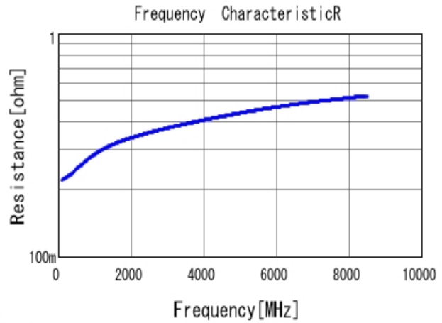
■ GRM0223C1H2R3CA03 R DCOV, 20degC
