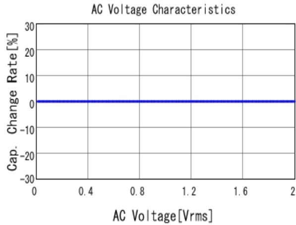
■ GRM0223C1H2R3CA03 C-AC Voltage capchange, DCOV, 20.0d
