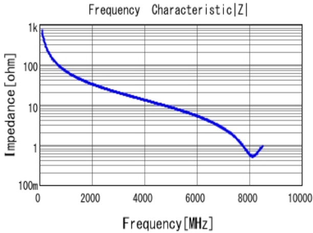
■ GRM0223C1H2R3CA03 |Z| DCOV, 20degC
