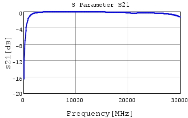
GRM0223C1H2R4WA03 S21 DCOV, 20degC
