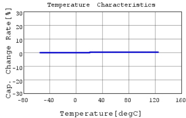
GRM0223C1H2R4WA03 C-Temp. capchange, DCOV, 1
