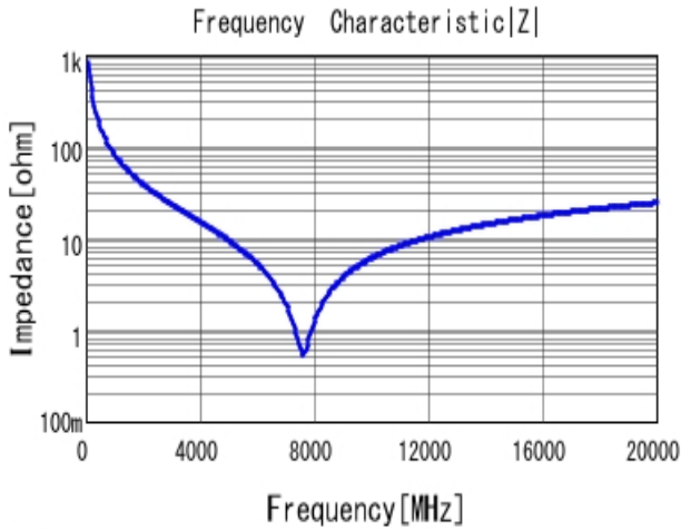
■ GRM0224C1H1R9WA03 |Z| DCOV, 20degC
