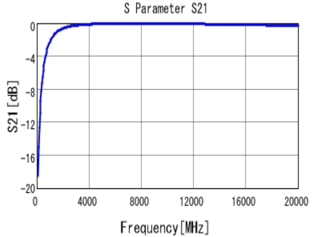
■ GRM0224C1H1R9WA03 S21 DCOV, 20degC
