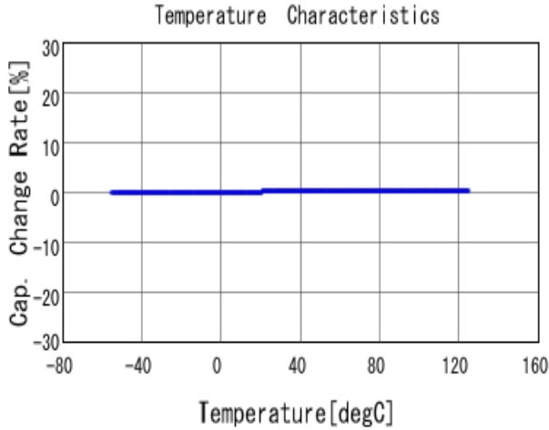
■ GRM0224C1H1R9WA03 C-Temp. capchange, DCOV, AC1Vrms
