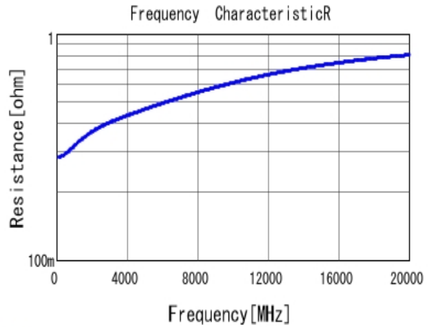
■ GRM0224C1H1R9WA03 R DCOV, 20degC
