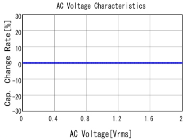
■ GRM0225C1H150JA03 C-AC Voltage capchange, DCOV, 25.0d
