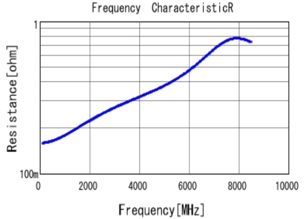
■ GRM0225C1H150JA03 R DCOV, 25degC
