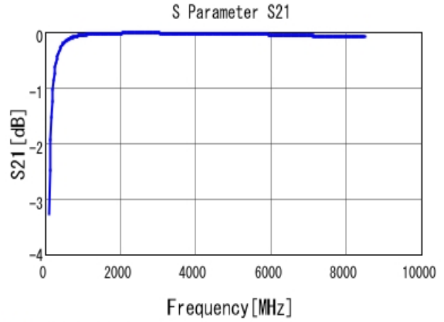
■ GRM0225C1H150JA03 S21 DCOV, 25degC
