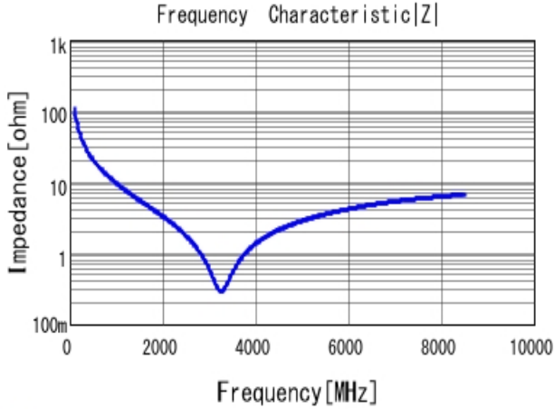
■ GRM0225C1H150JA03 |Z| DCOV, 25degC
