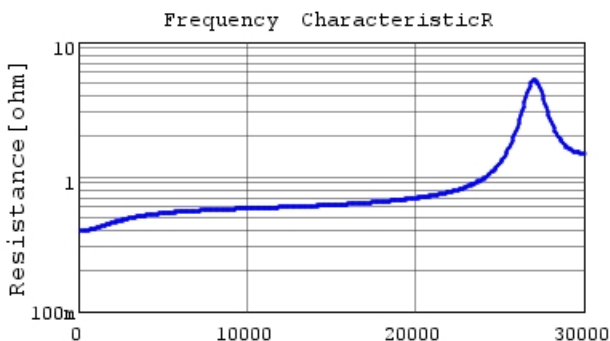
GRM0225C1H1R3WA03 R DCOV,25degC
