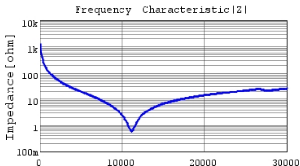
GRM0225C1H1R3WA03 |Z| DCOV,25degC
