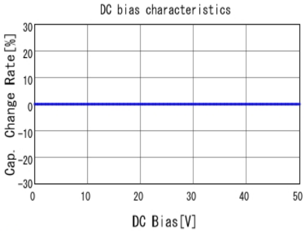
■ GRM0225C1H4R5BA03 C-DC bias capchange, 25.0degC, AC1V
