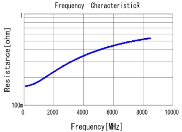
■ GRM0225C1H4R5BA03 R DCOV, 25degC
