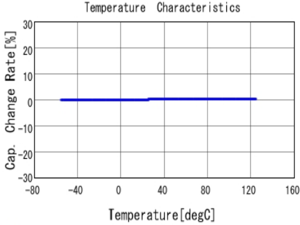
■ GRM0225C1H4R5BA03 C-Temp. capchange, DCOV, AC1Vrms
