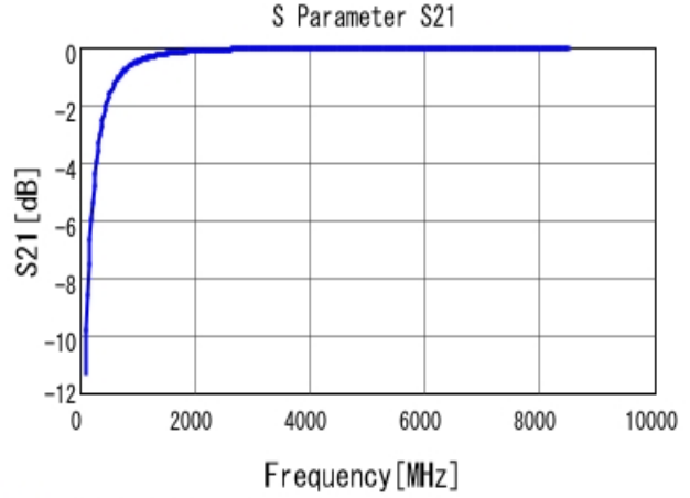
■ GRM0225C1H4R5BA03 S21 DCOV, 25degC
