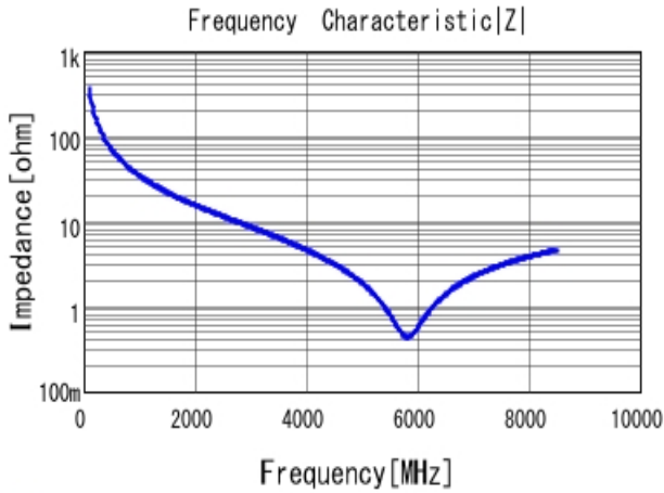
■ GRM0225C1H4R5BA03 |Z| DCOV, 25degC
